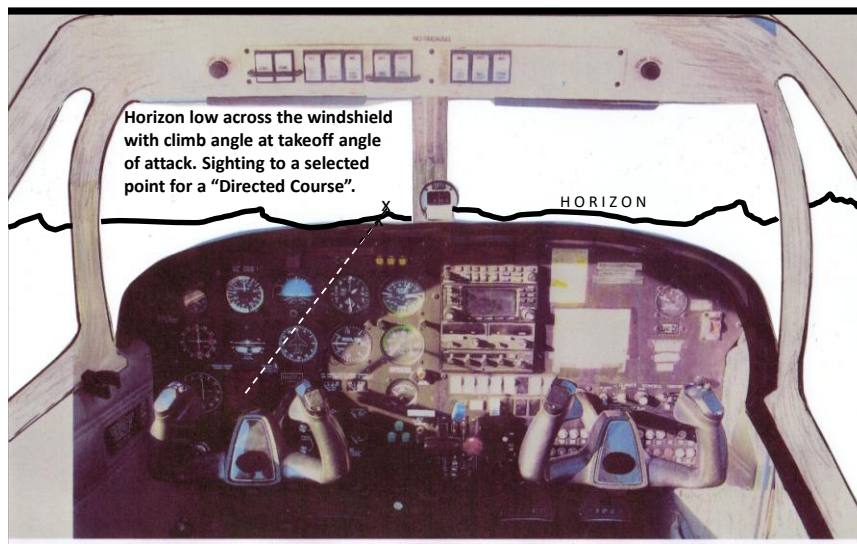
"DIRECTED COURSE" VISUAL REFERENCE FLIGHT TAKEOFF AND CLIMBING WINGS LEVEL FLIGHT
